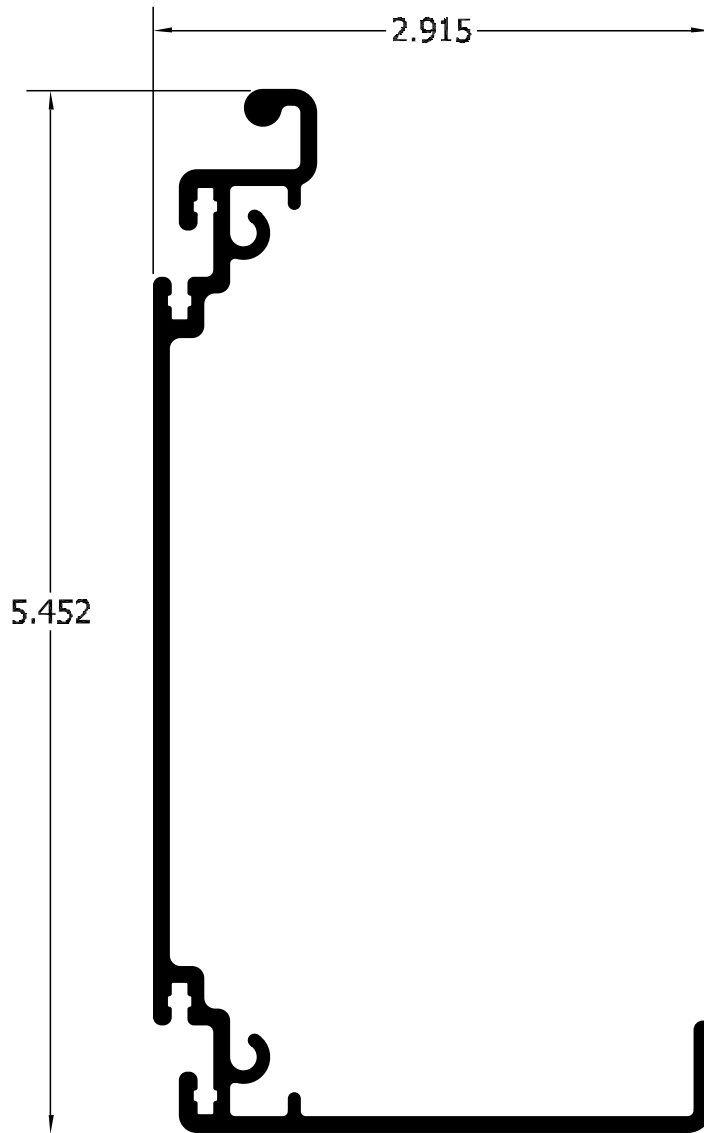
5" Narrow Access Raceway - Back Part#1962N
